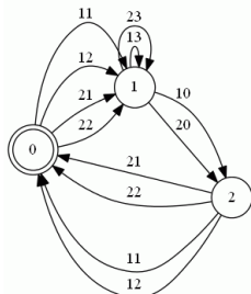
Fig. 13. The feasible supervisor for the guide way \Sigma_{uo} = \{13, 23\} ,
