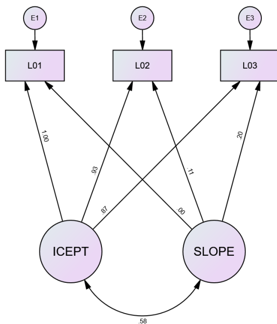
Figure 2 LGCM Model with Standardized Estimates
